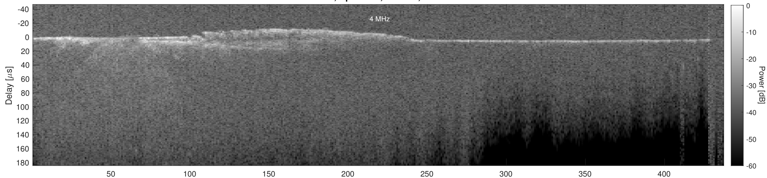
Orbit 5401, Cluttergram
