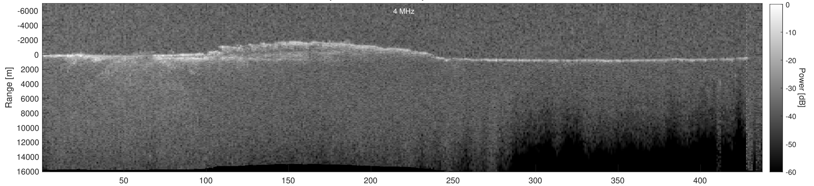
Orbit 5401, Depth-Corrected Cluttergram
