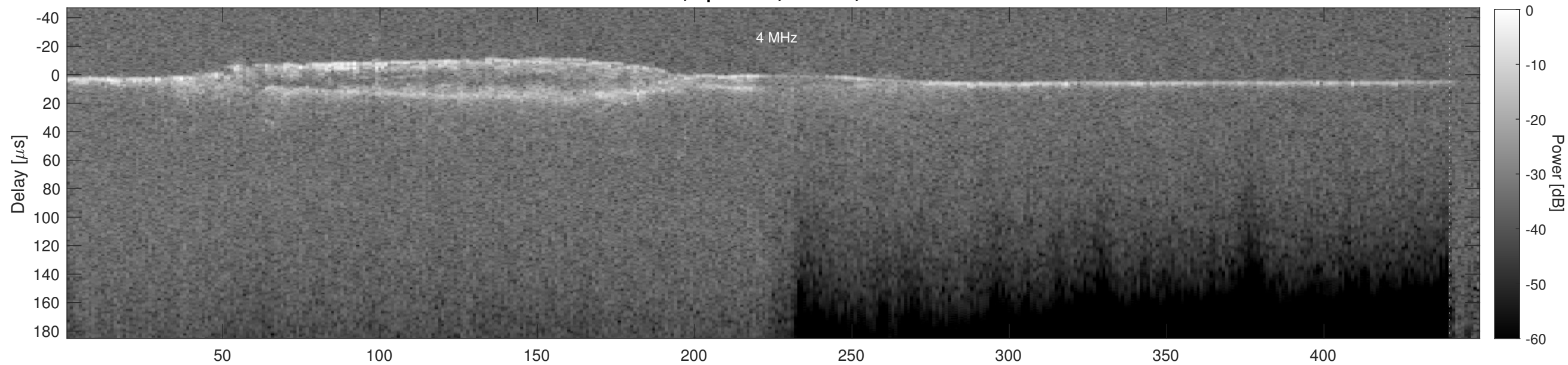
Orbit 5402, Cluttergram
