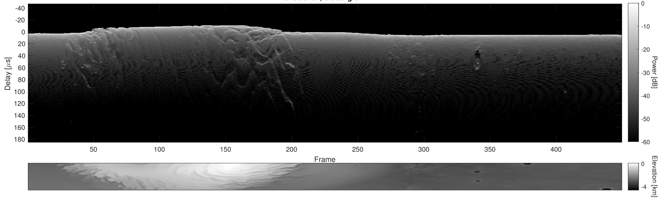
Orbit 5402, Cluttergram
