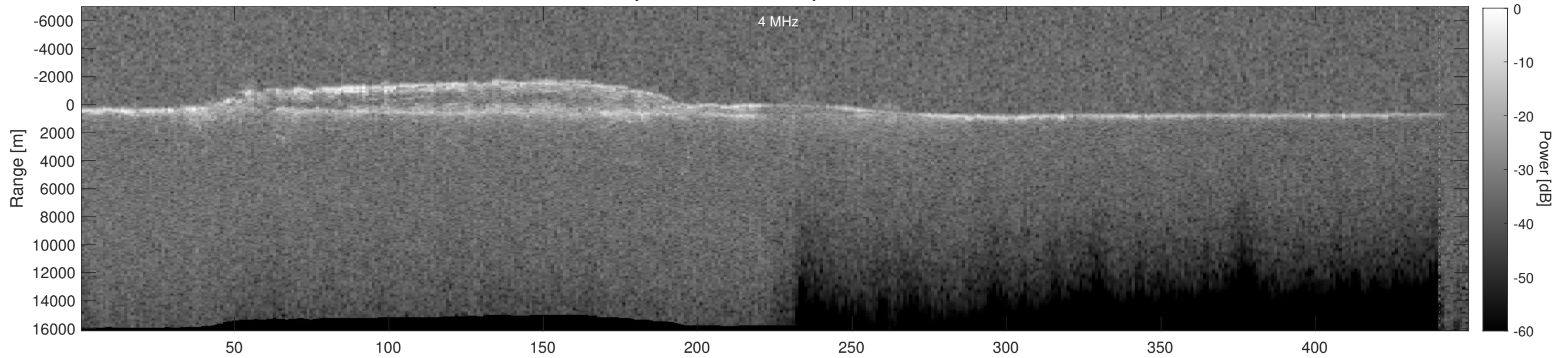
Orbit 5402, Depth-Corrected Cluttergram
