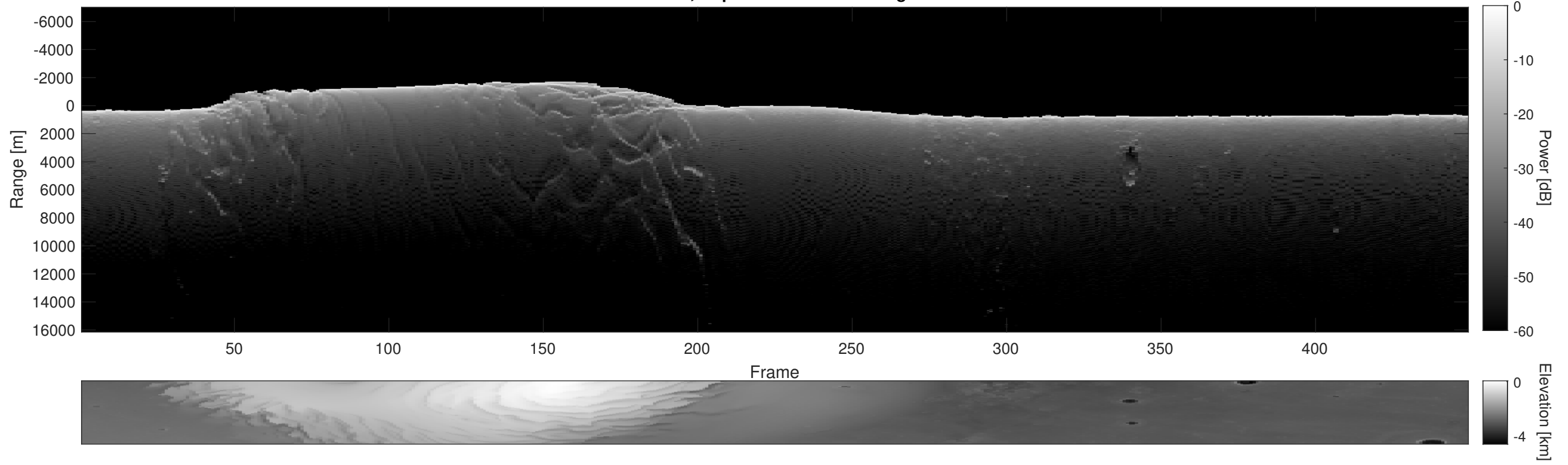
Orbit 5402, Depth-Corrected Cluttergram
