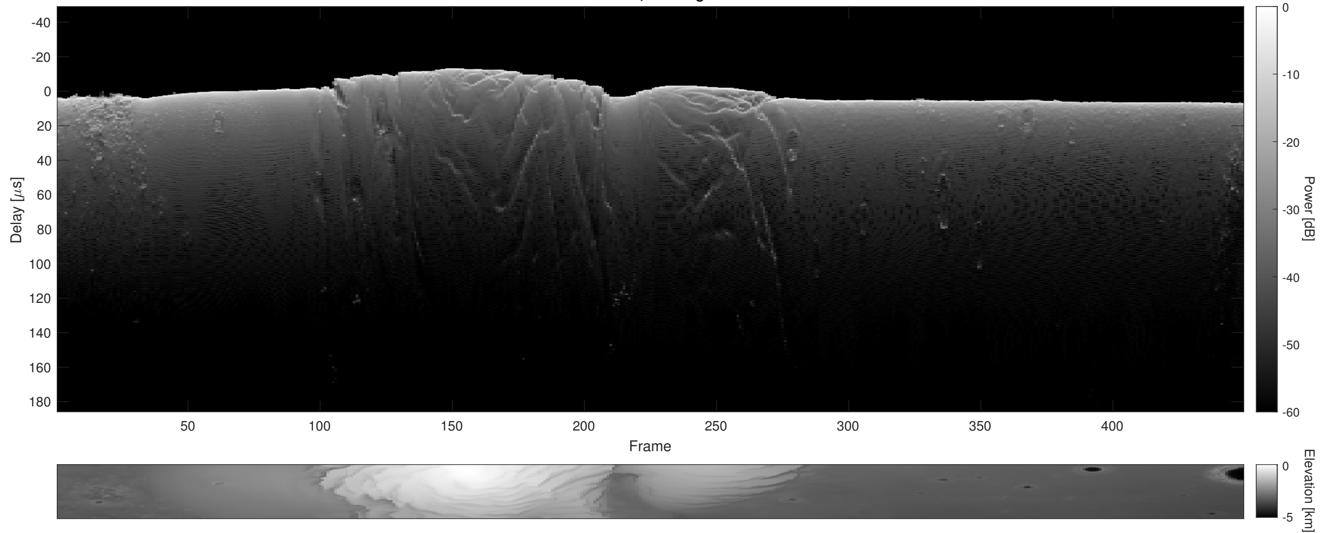
Orbit 5404, Cluttergram
