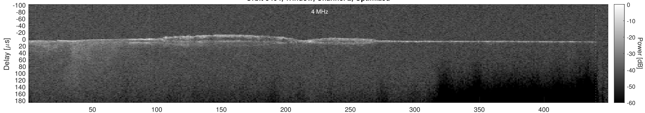
Orbit 5404, Cluttergram
