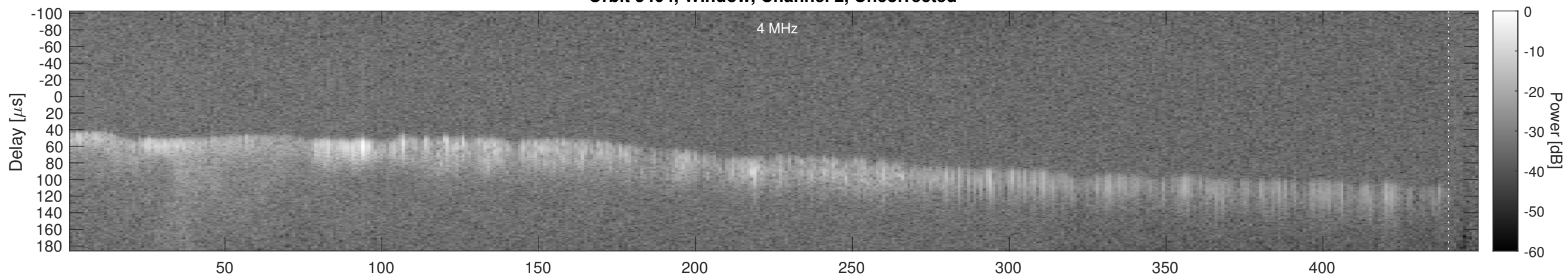
Orbit 5404, Window, Channel 2, Chapman
