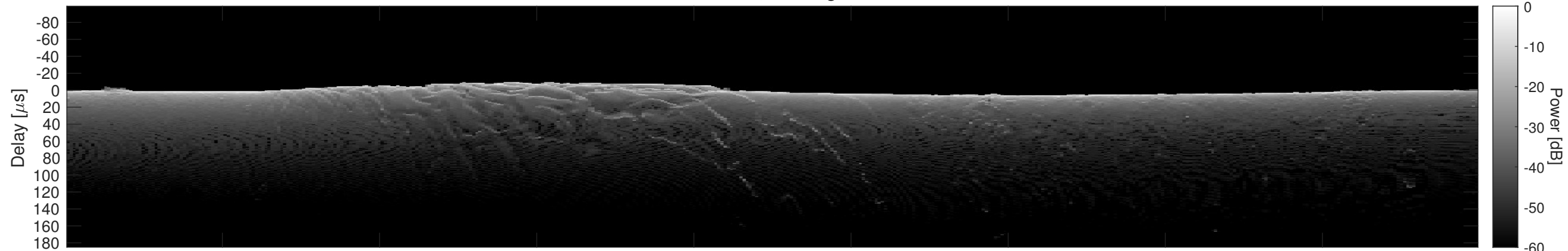
Orbit 5405, Cluttergram
