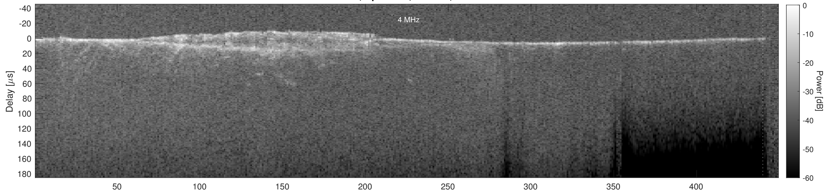
Orbit 5405, Cluttergram
