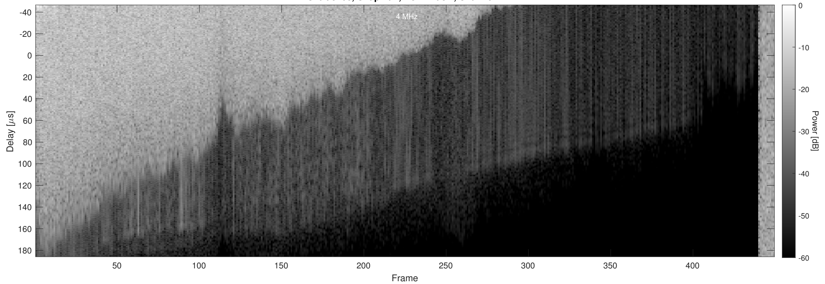
Orbit 5406, Chapman, No Window, Channel 2
