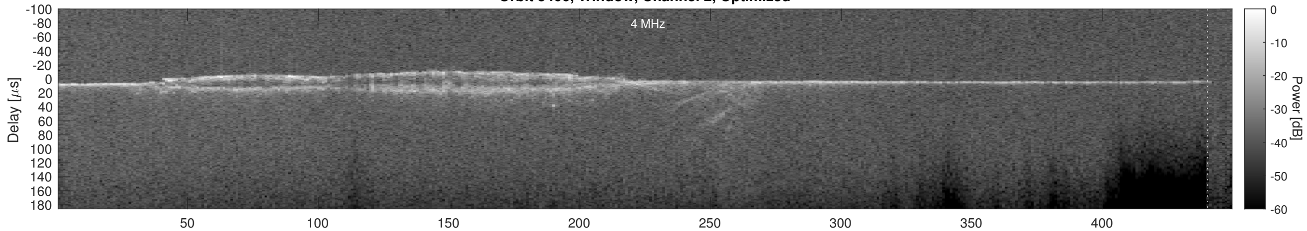
Orbit 5406, Cluttergram
