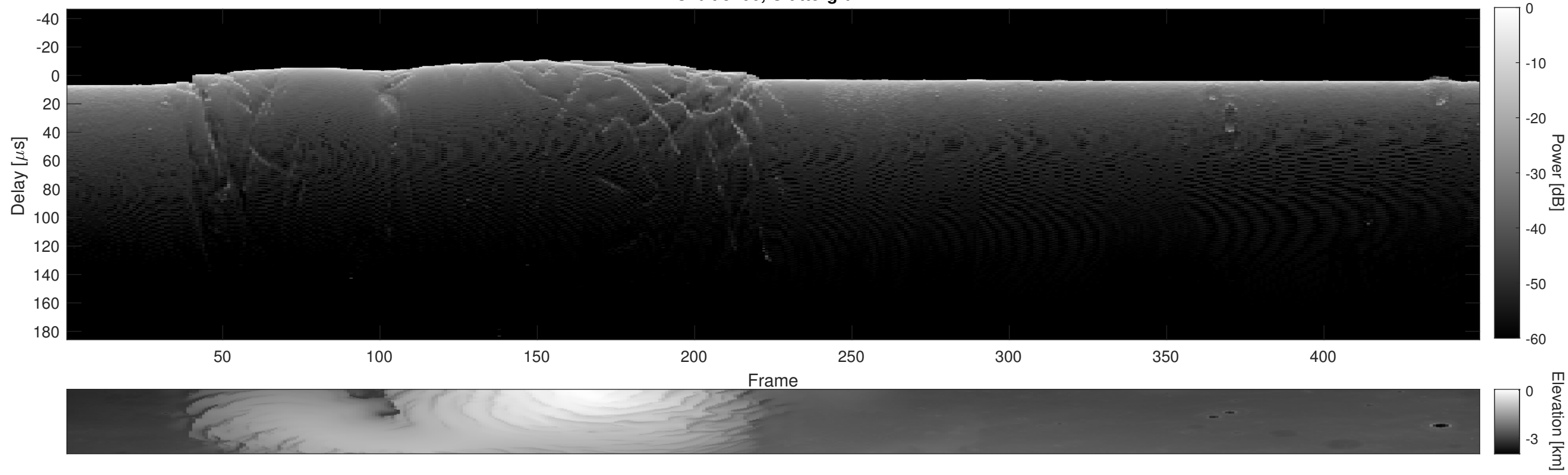
Orbit 5406, Cluttergram
