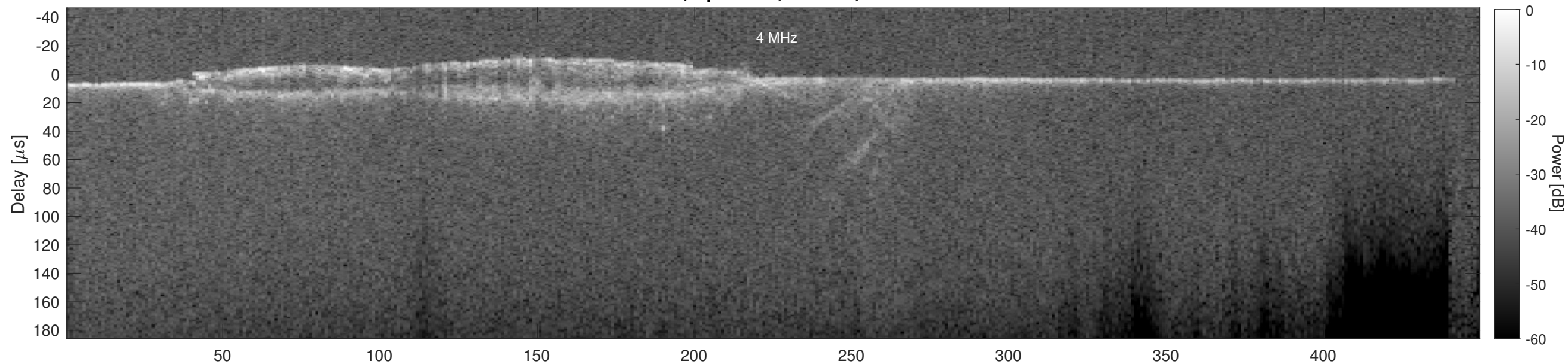
Orbit 5406, Cluttergram
