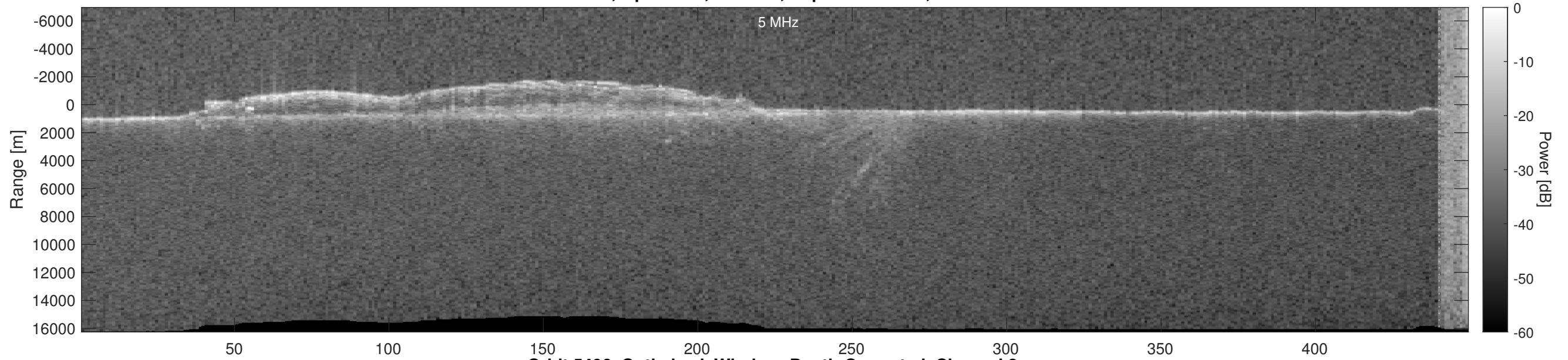
Orbit 5406, Optimized, Window, Depth-Corrected, Channel 2
