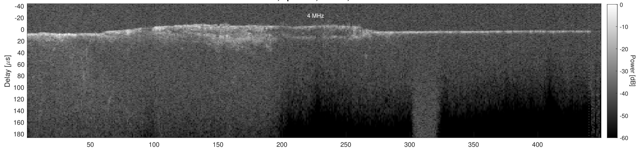
Orbit 5407, Cluttergram
