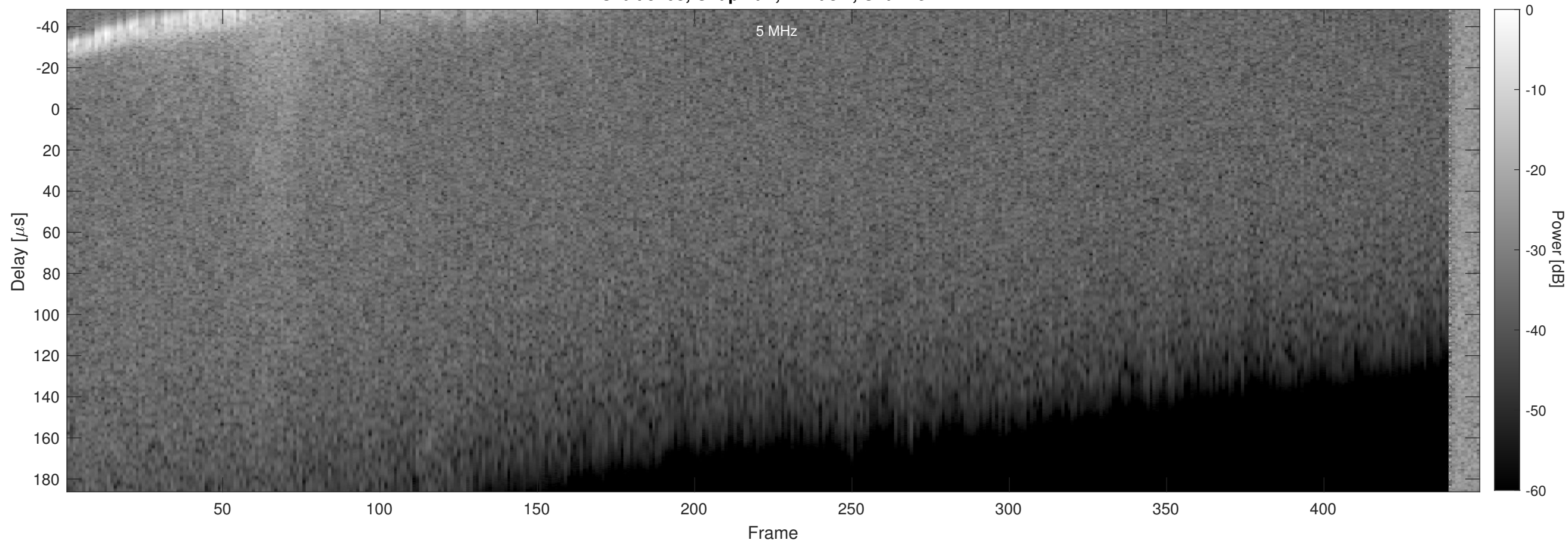
Orbit 5408, Chapman, Window, Channel 2
