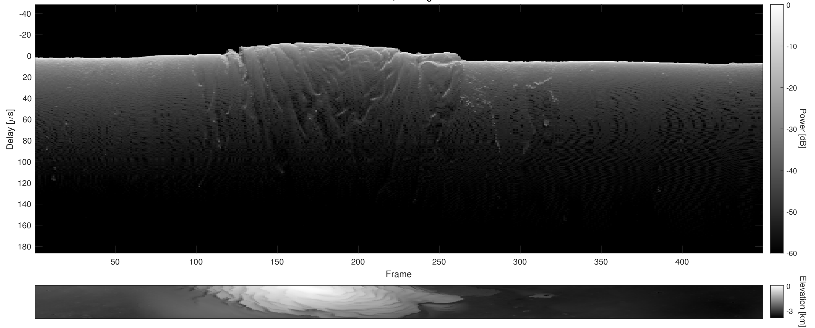
Orbit 5408, Cluttergram
