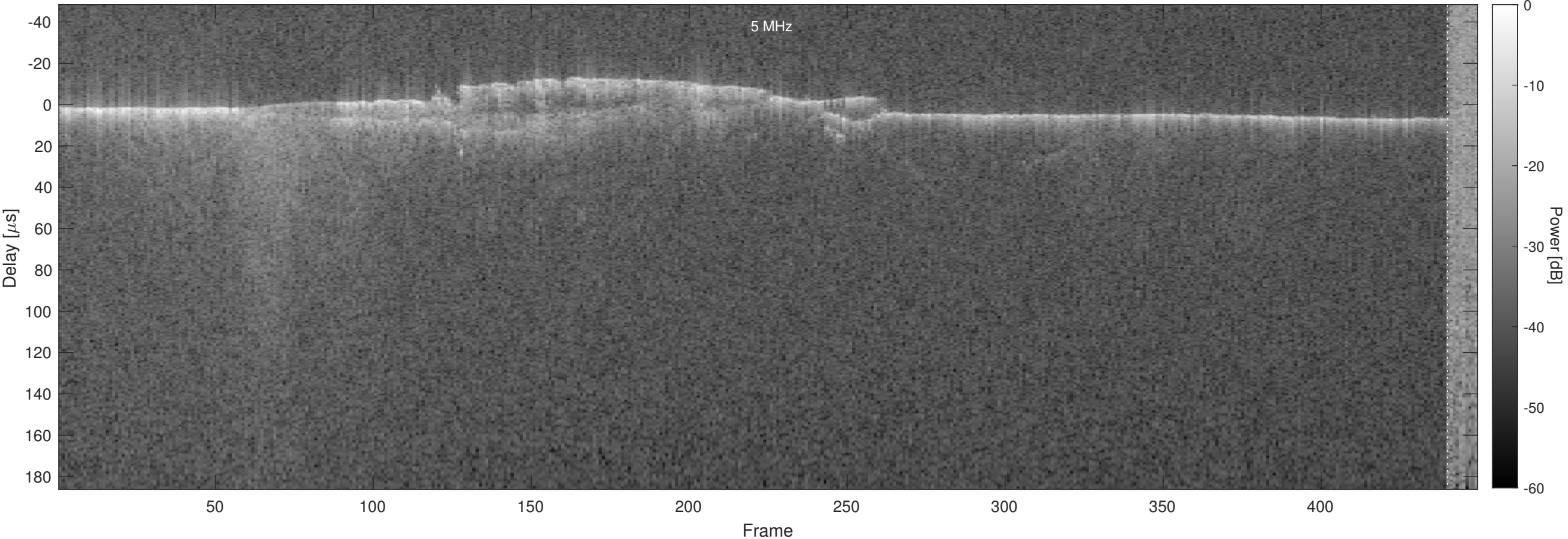
Orbit 5408, Optimized, No Window, Channel 2
