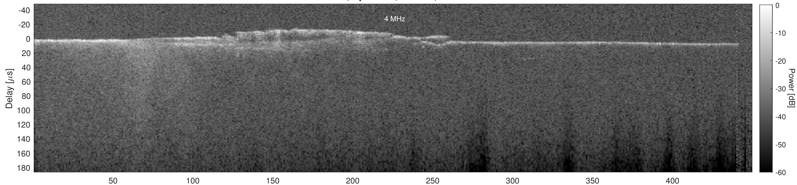
Orbit 5408, Cluttergram
