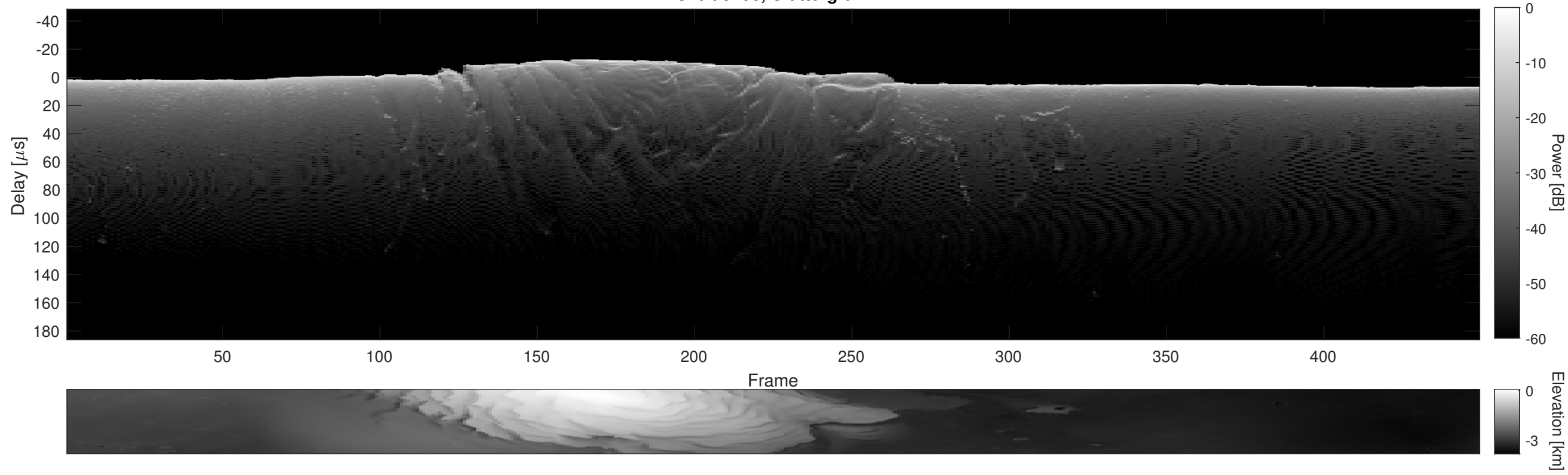
Orbit 5408, Cluttergram
