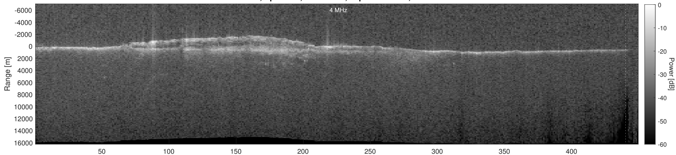
Orbit 5409, Depth-Corrected Cluttergram
