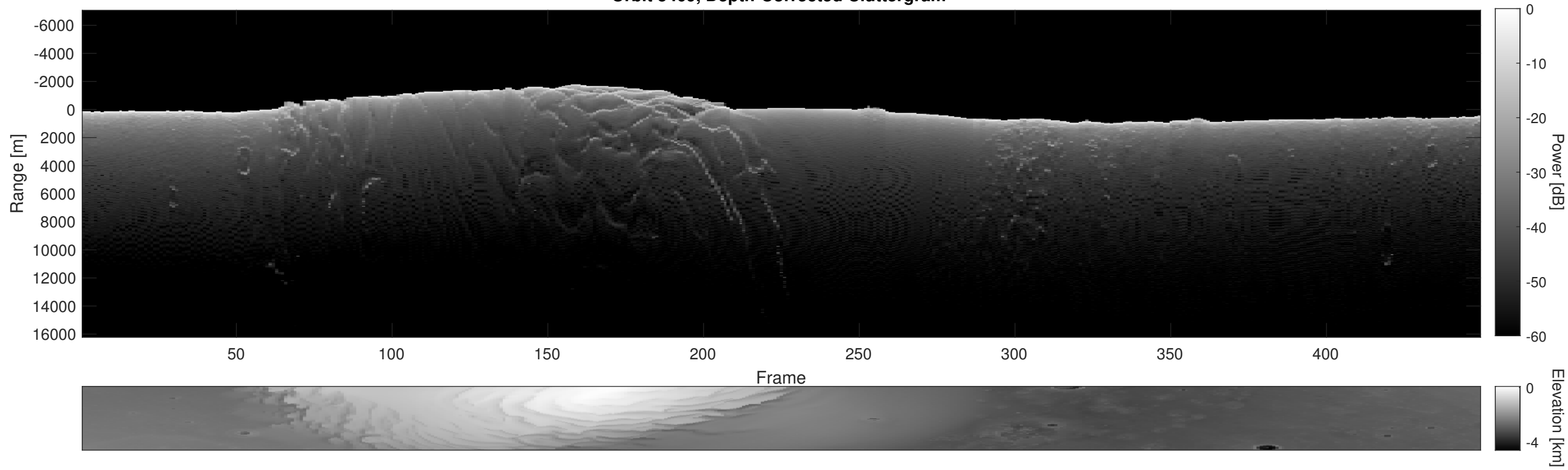
Orbit 5409, Depth-Corrected Cluttergram
