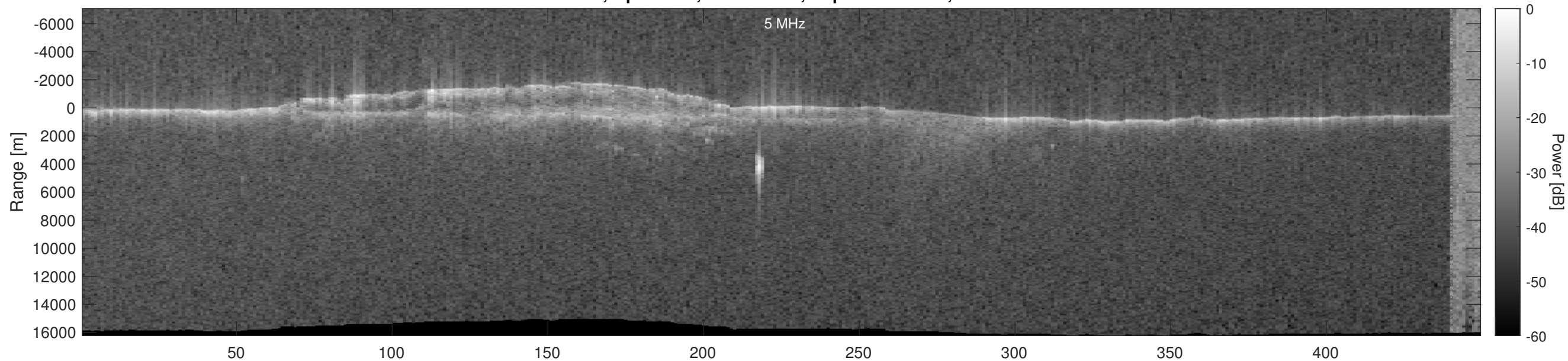
Orbit 5409, Optimized, No Window, Depth-Corrected, Channel 2
