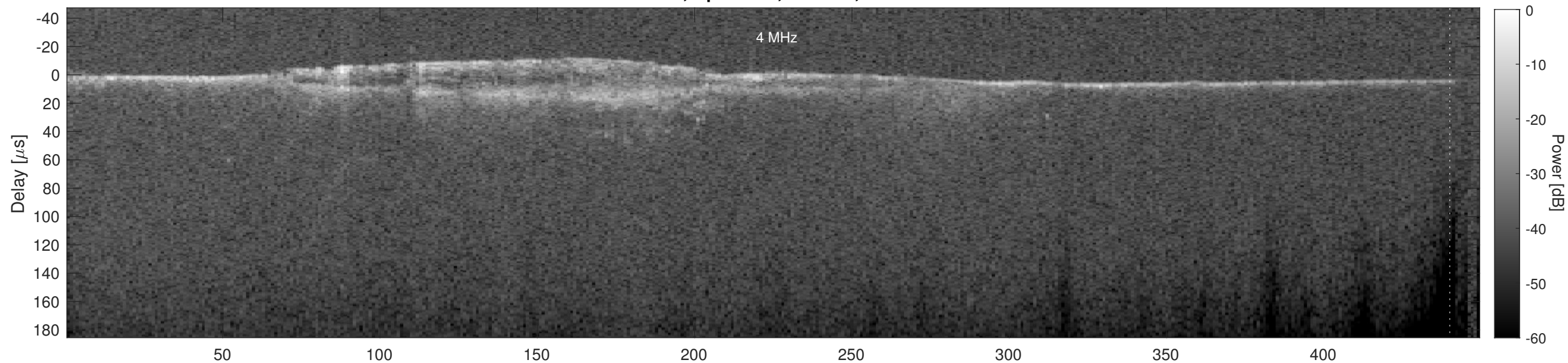
Orbit 5409, Cluttergram
