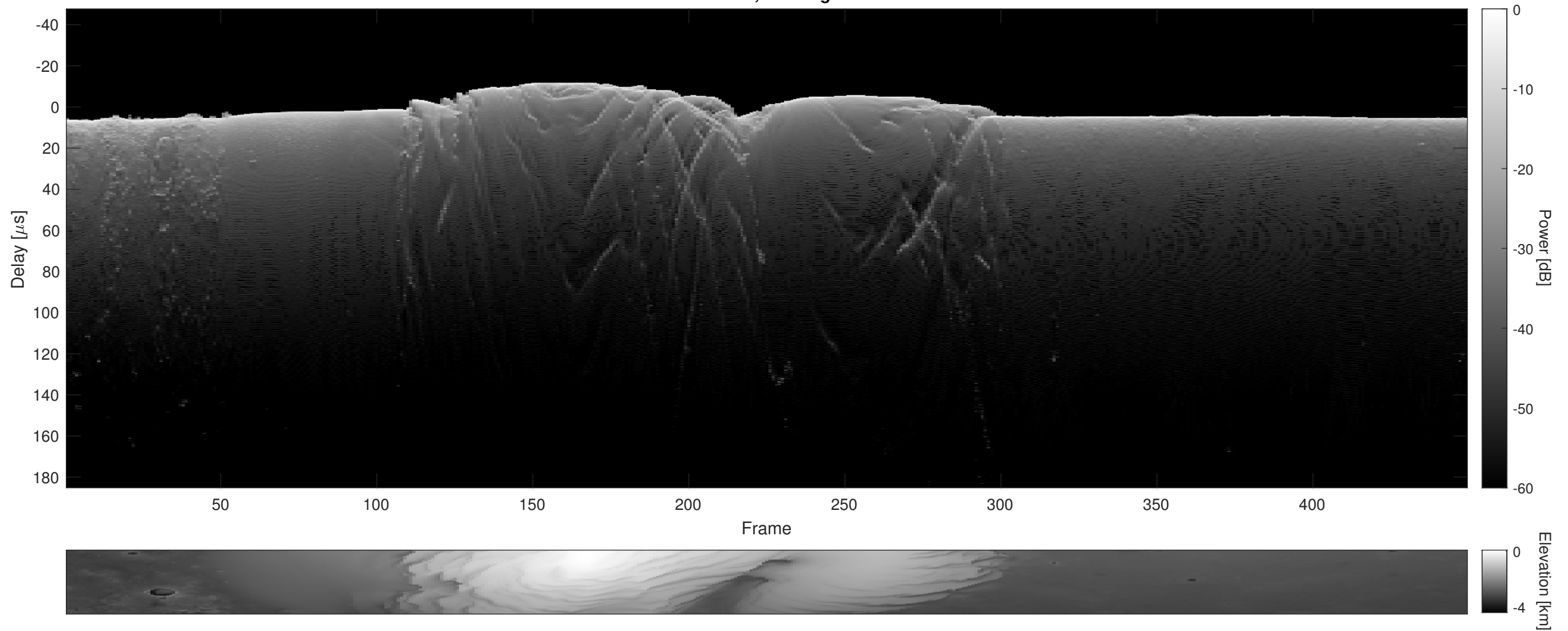
Orbit 5411, Cluttergram
