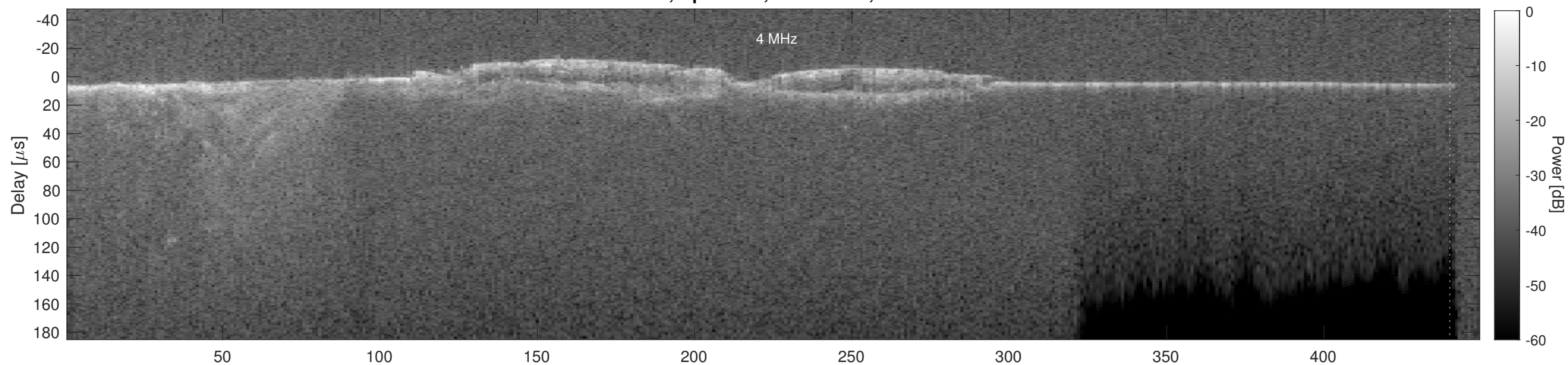
Orbit 5411, Cluttergram
