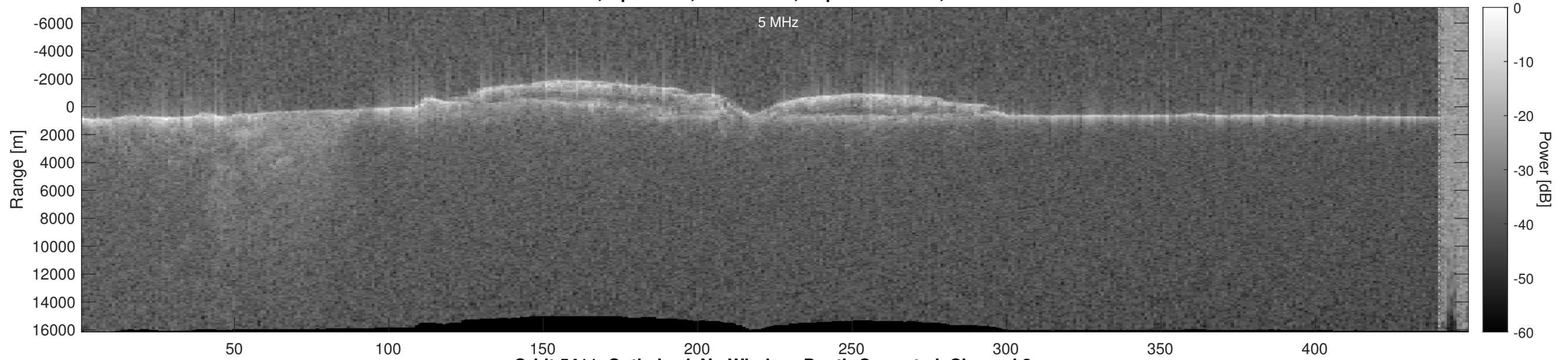
Orbit 5411, Optimized, No Window, Depth-Corrected, Channel 2
