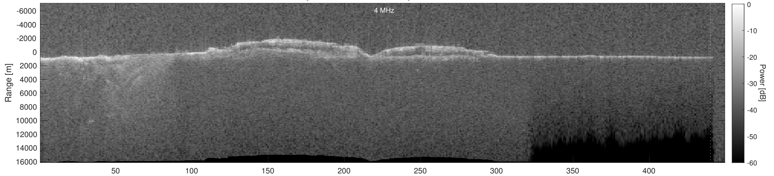
Orbit 5411, Depth-Corrected Cluttergram
