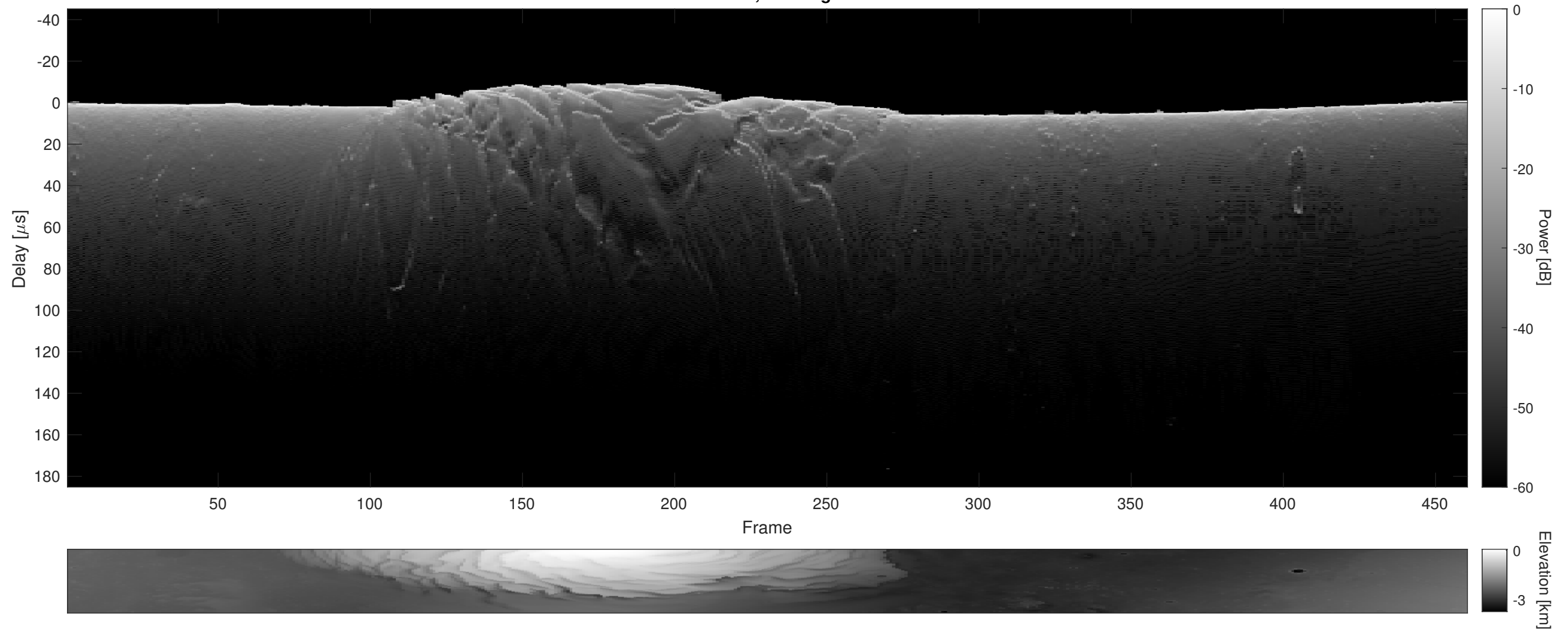
Orbit 5412, Cluttergram
