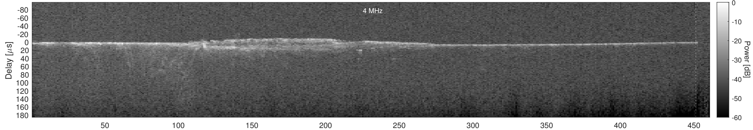
Orbit 5412, Cluttergram
