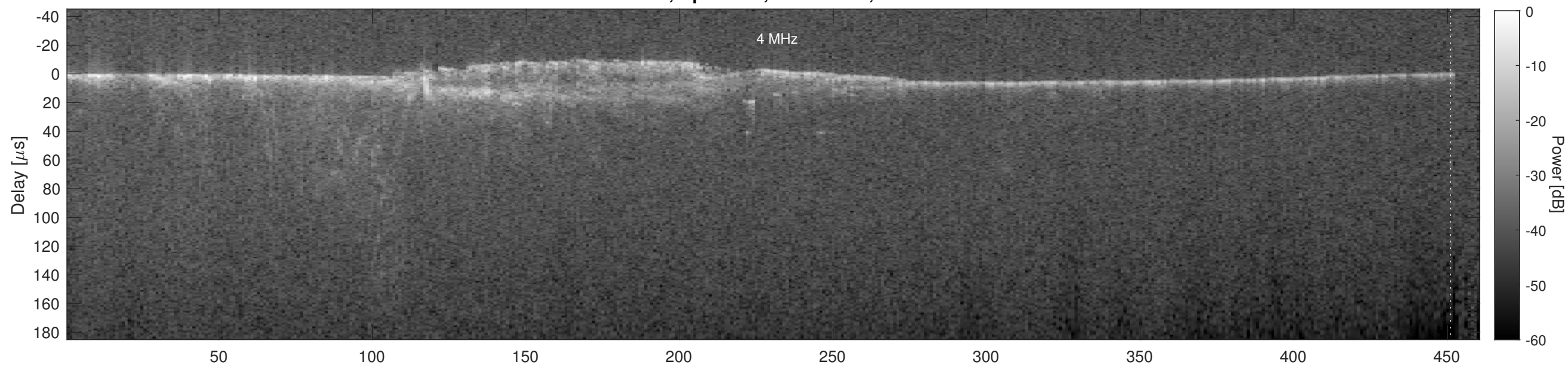
Orbit 5412, Cluttergram
