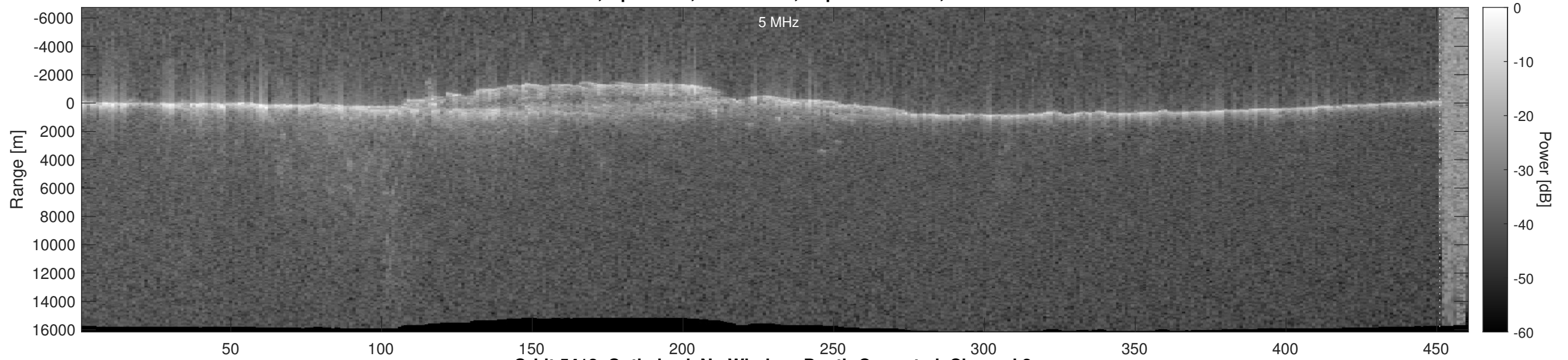
Orbit 5412, Optimized, No Window, Depth-Corrected, Channel 2
