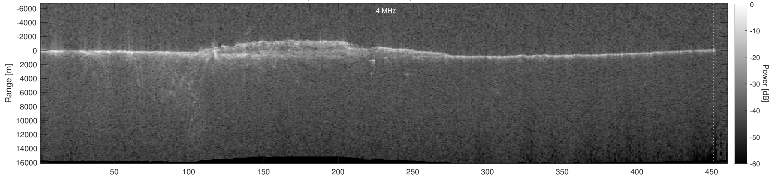
Orbit 5412, Depth-Corrected Cluttergram
