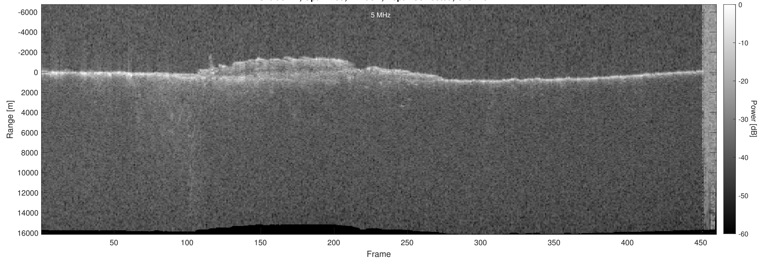
Orbit 5412, Optimized, Window, Depth-Corrected, Channel 2
