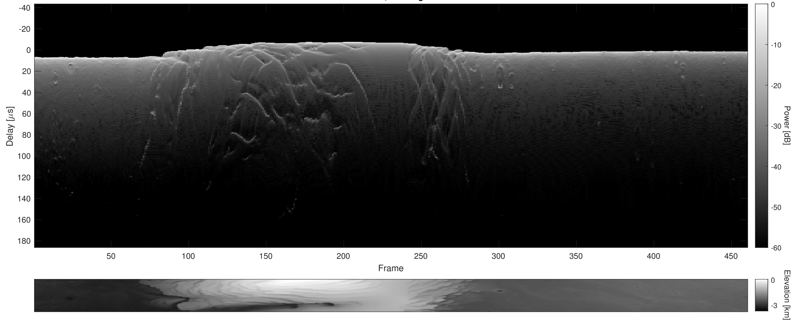
Orbit 5414, Cluttergram
