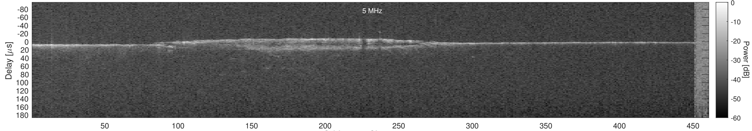
Orbit 5414, Cluttergram
