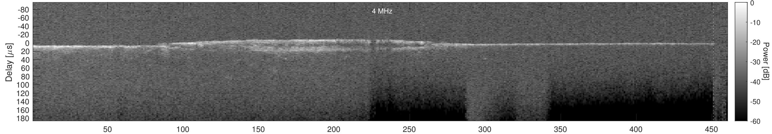
Orbit 5414, Cluttergram
