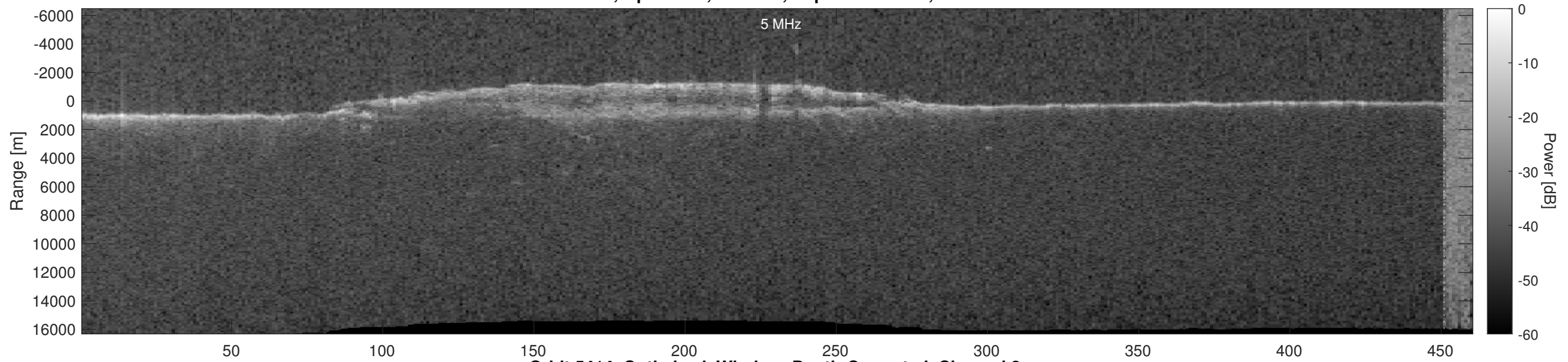
Orbit 5414, Optimized, Window, Depth-Corrected, Channel 2
