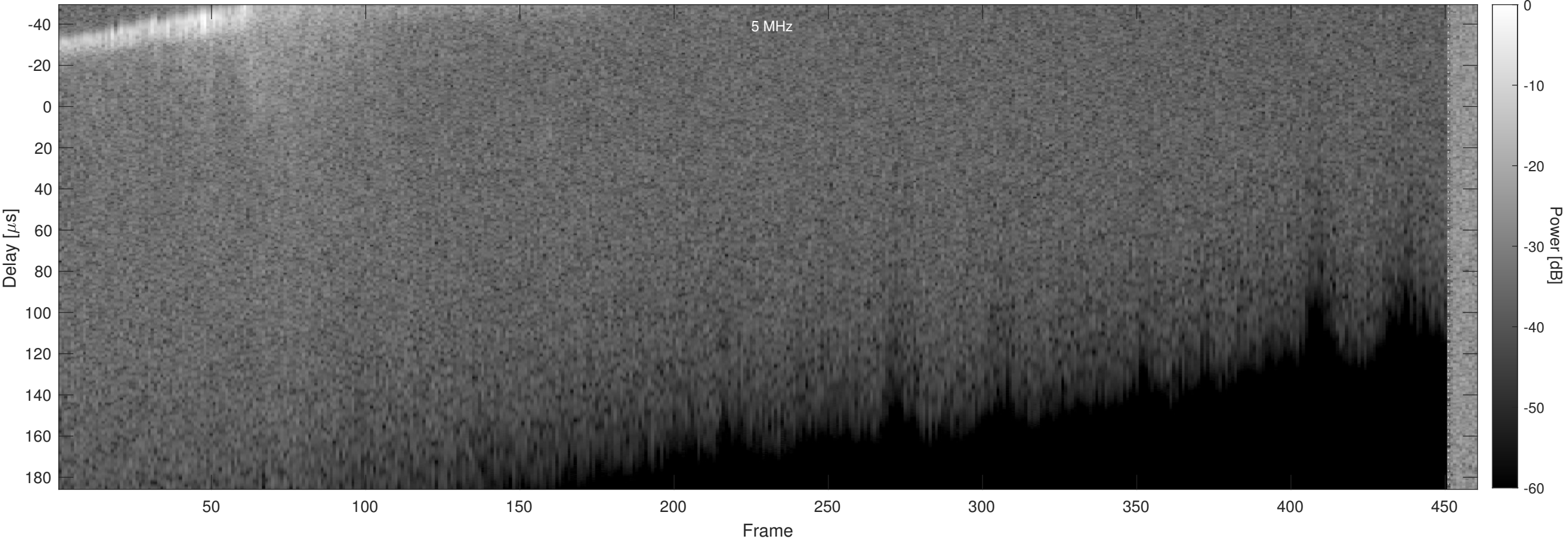
Orbit 5415, Chapman, Window, Channel 2
