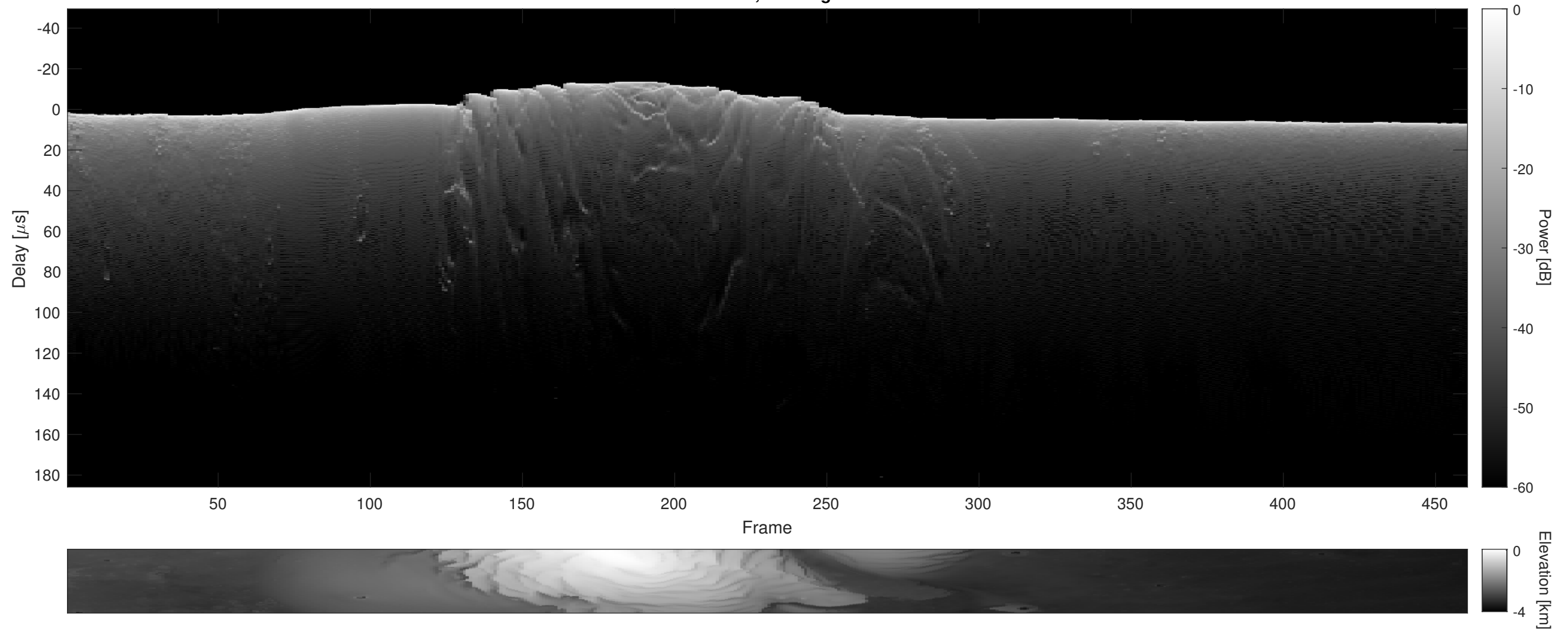
Orbit 5415, Cluttergram
