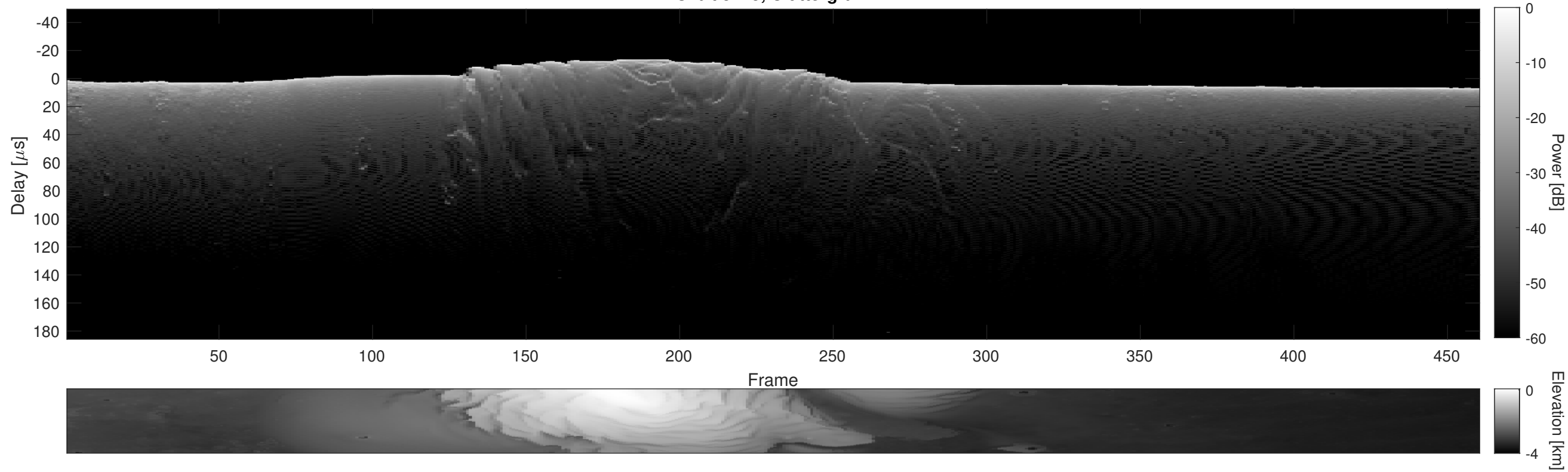
Orbit 5415, Cluttergram
