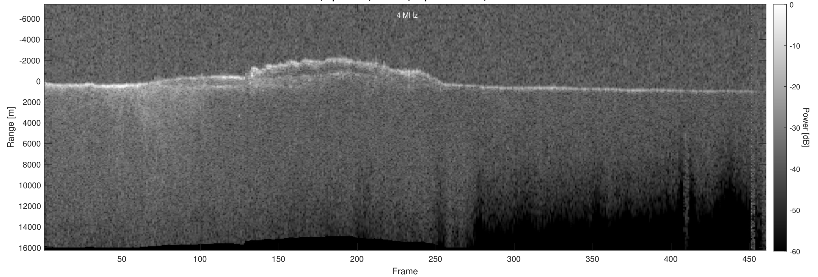
Orbit 5415, Optimized, Window, Depth-Corrected, Channel 2
