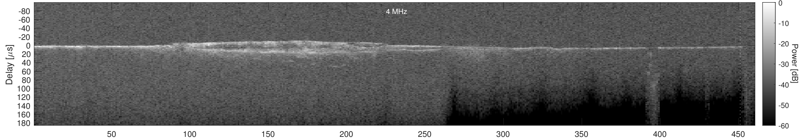
Orbit 5416, Cluttergram
