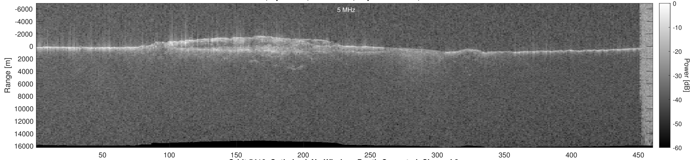
Orbit 5416, Optimized, No Window, Depth-Corrected, Channel 2
