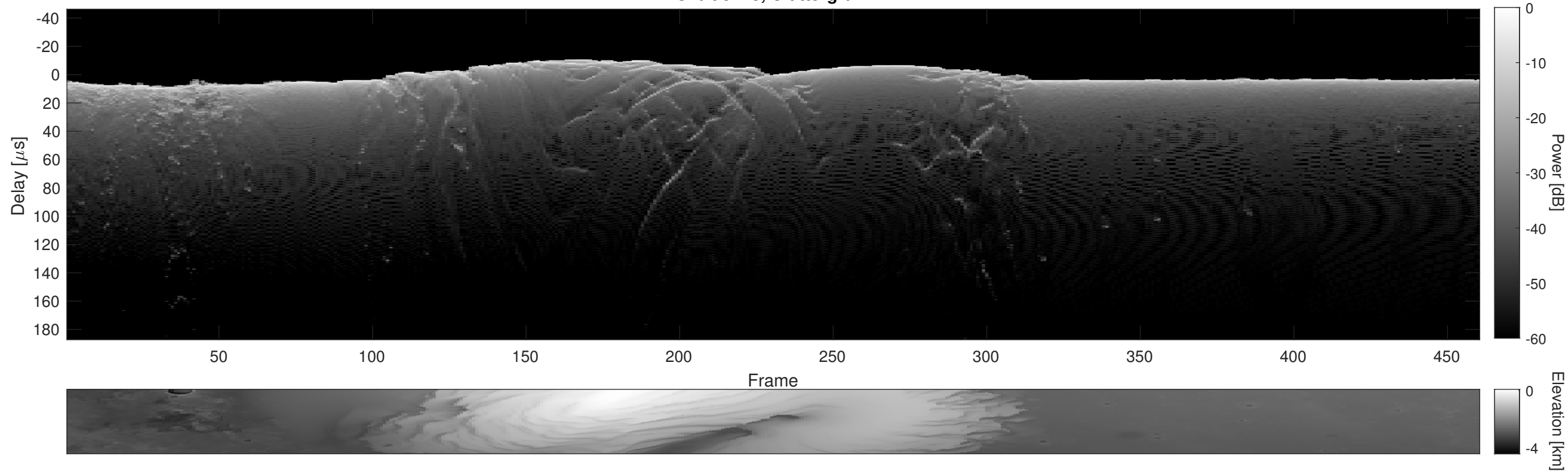
Orbit 5418, Cluttergram
