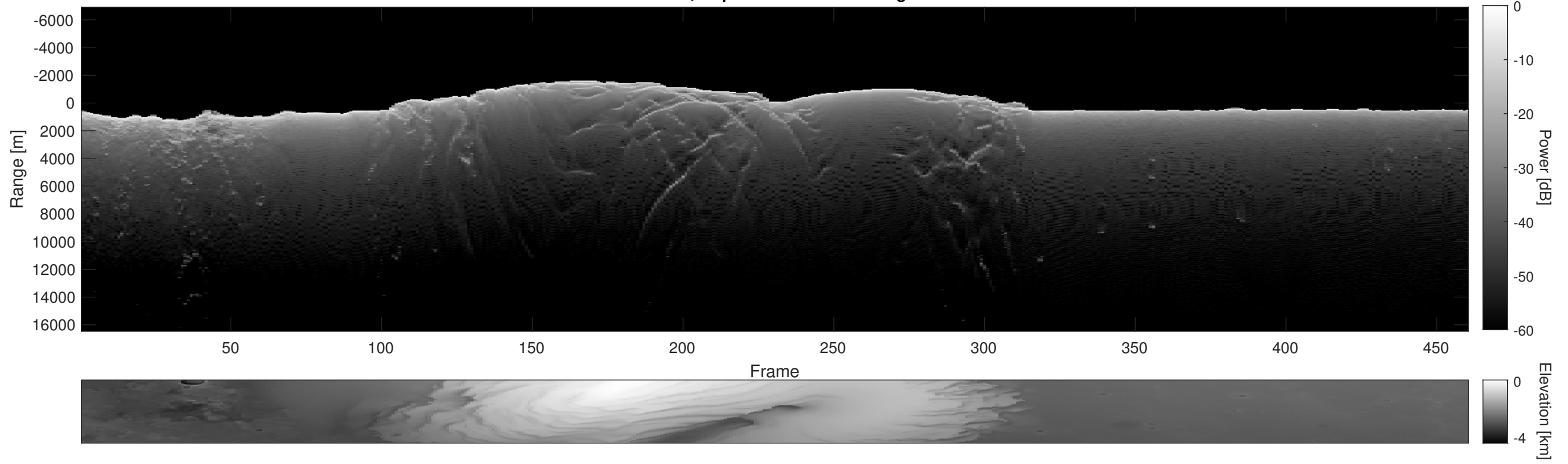
Orbit 5418, Depth-Corrected Cluttergram
