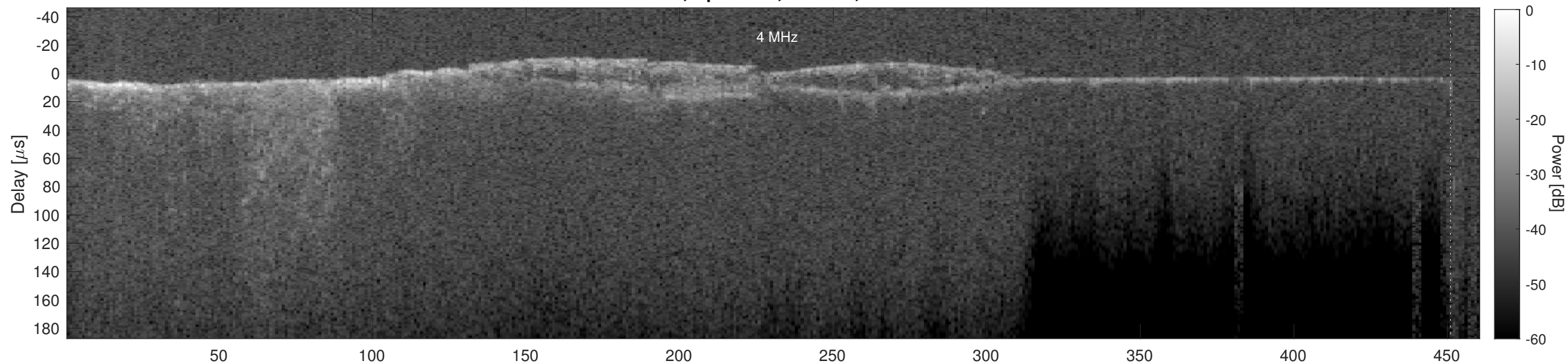
Orbit 5418, Cluttergram
