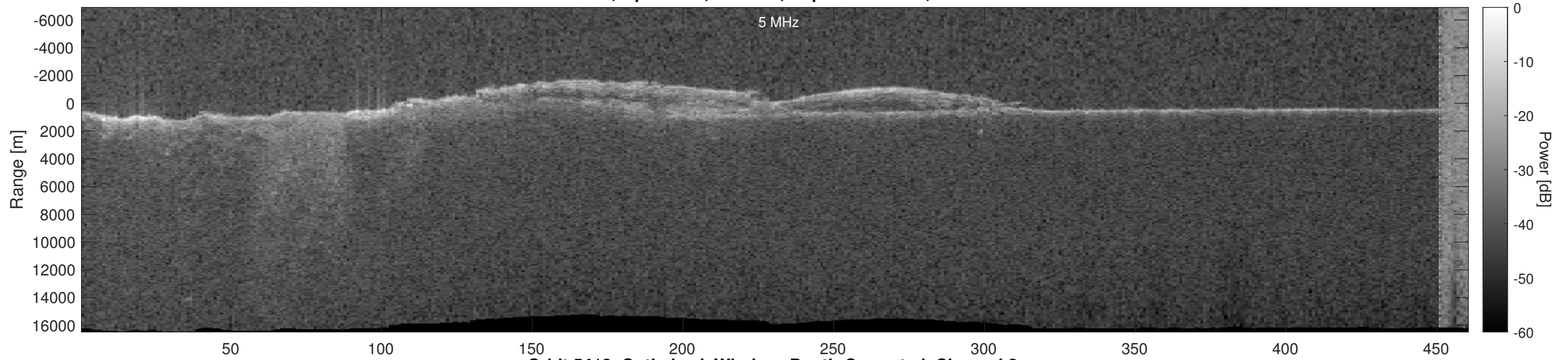
Orbit 5418, Optimized, Window, Depth-Corrected, Channel 2
