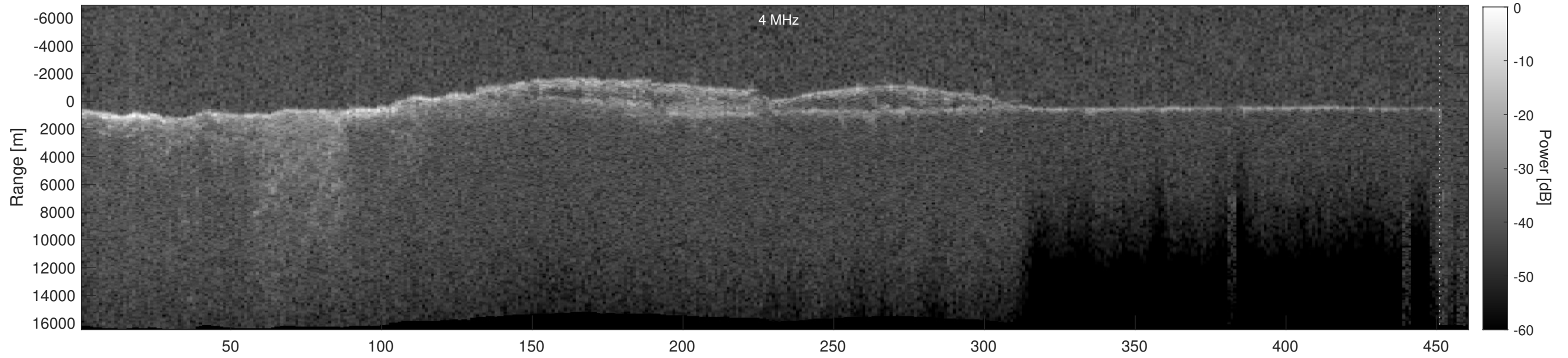
Orbit 5418, Depth-Corrected Cluttergram
