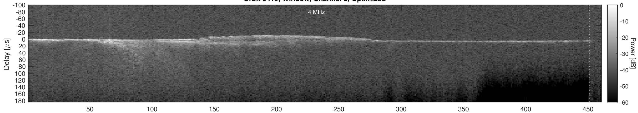
Orbit 5419, Cluttergram
