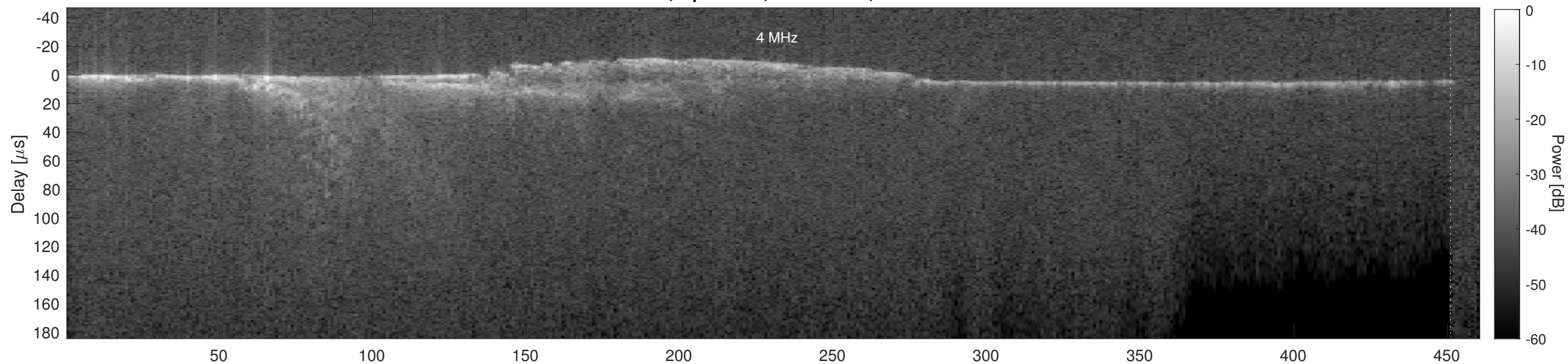
Orbit 5419, Cluttergram
