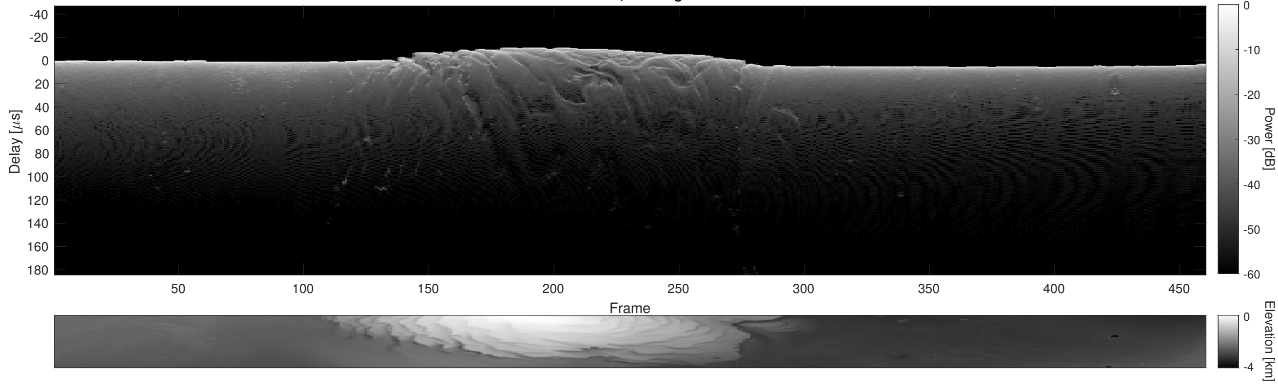
Orbit 5419, Cluttergram
