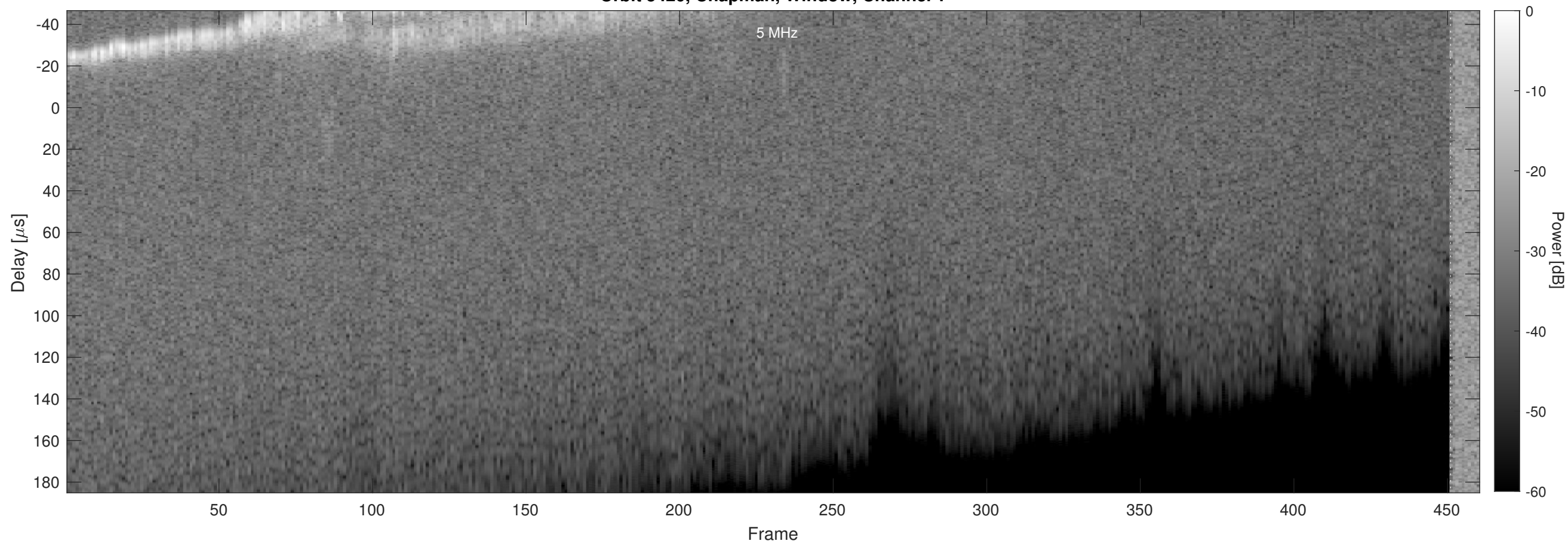
Orbit 5420, Chapman, Window, Channel 2
