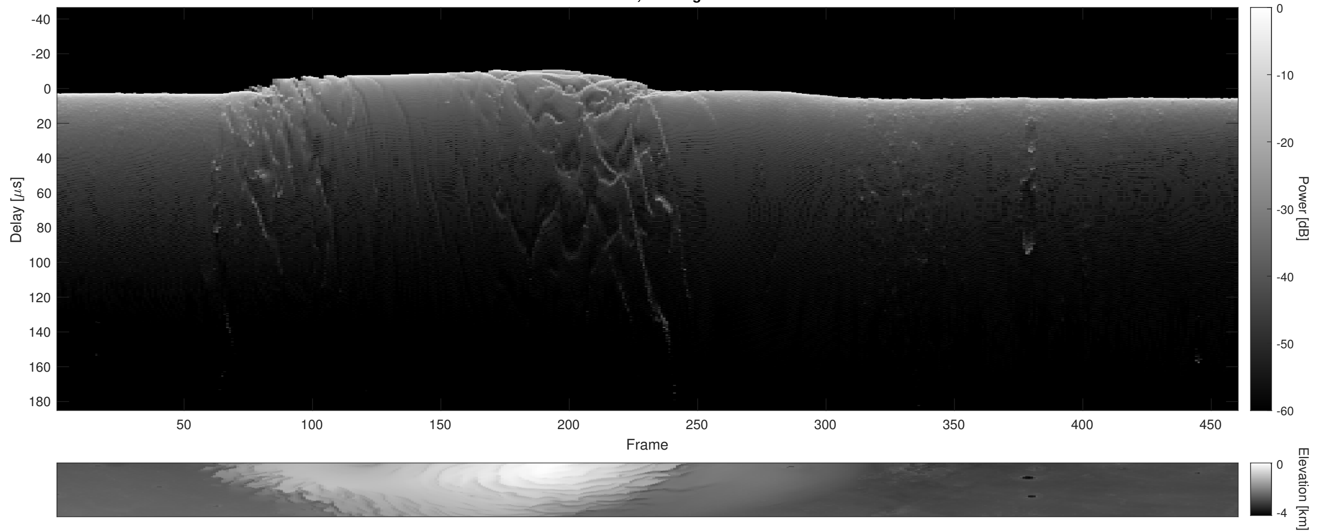
Orbit 5420, Cluttergram
