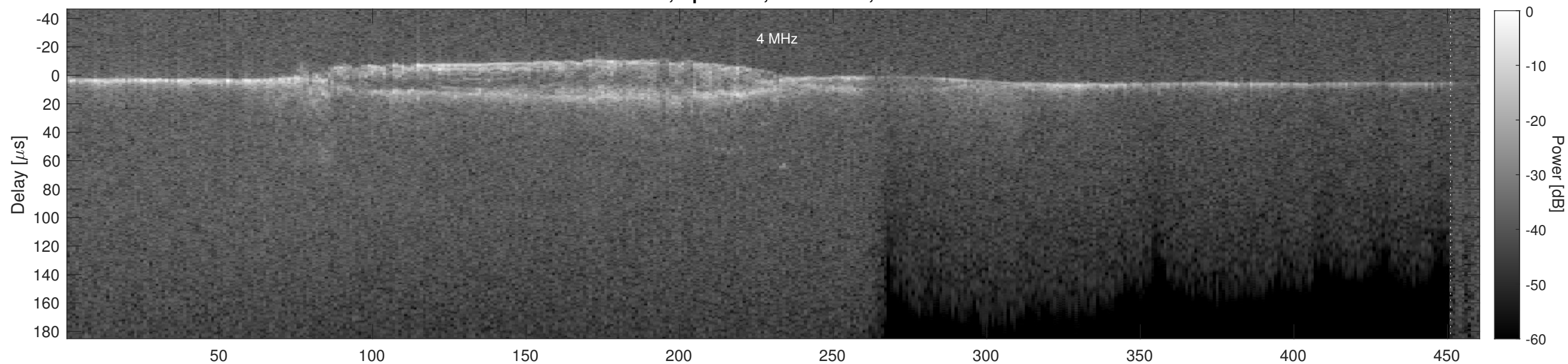
Orbit 5420, Cluttergram
