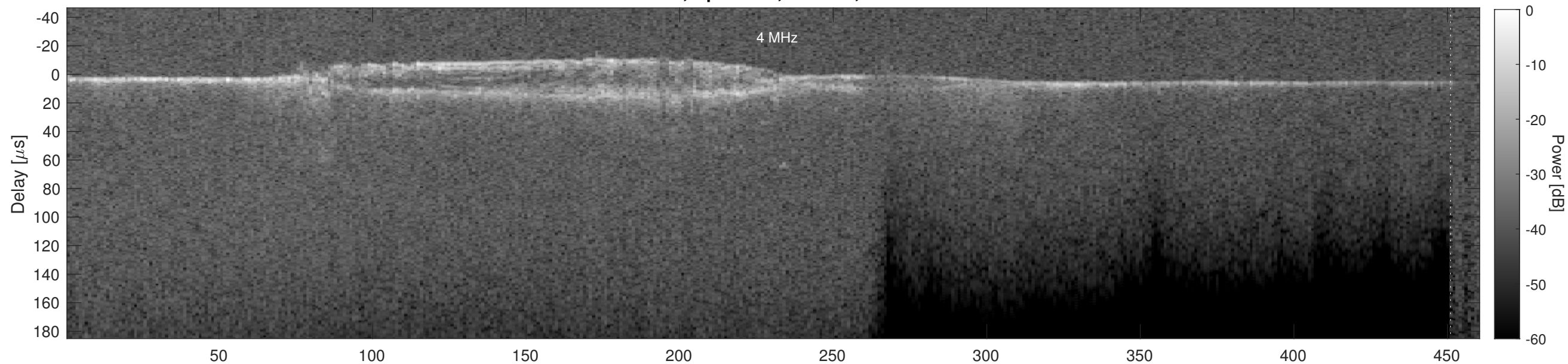
Orbit 5420, Cluttergram
