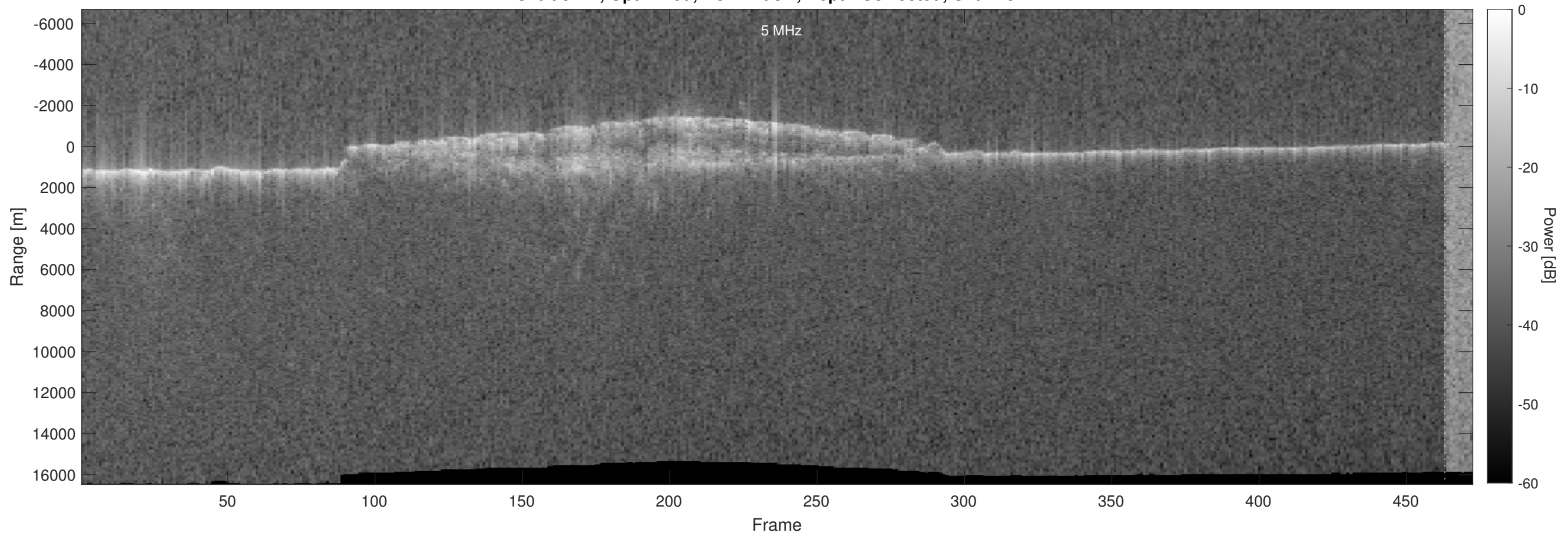
Orbit 5421, Optimized, No Window, Depth-Corrected, Channel 2
