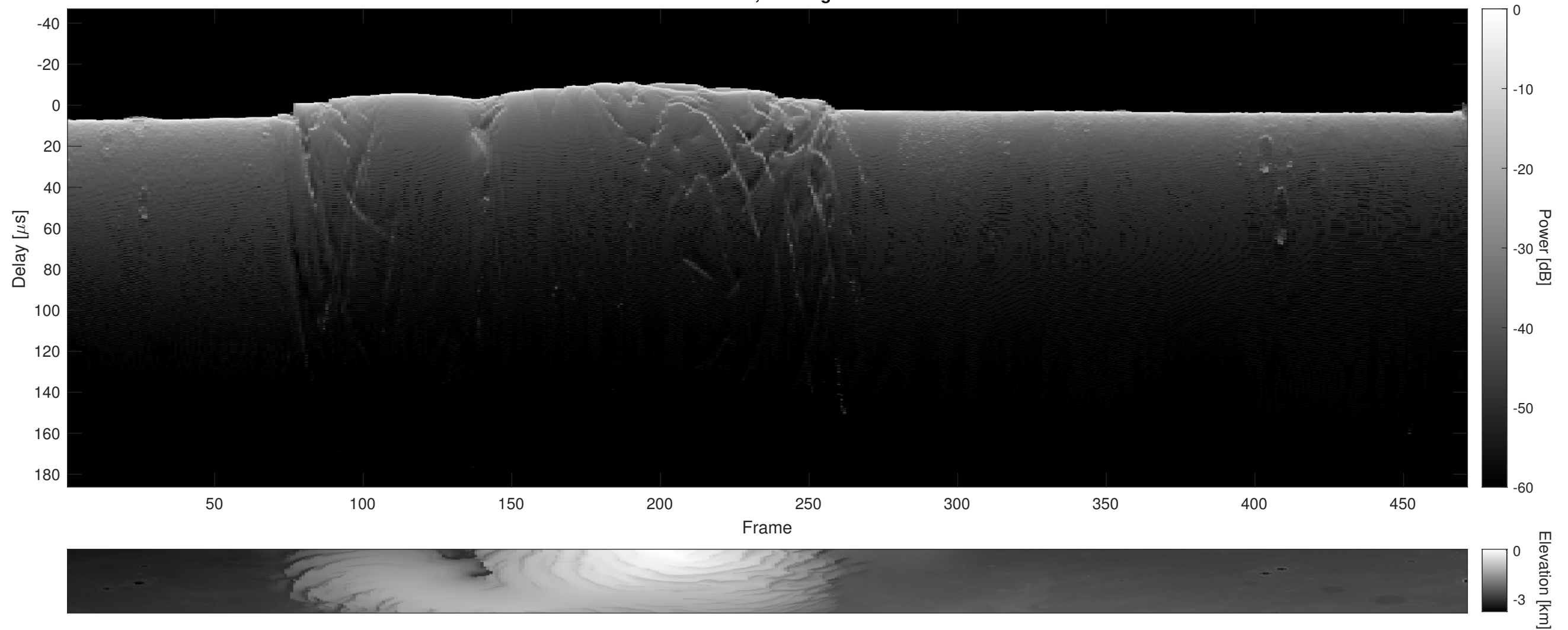
Orbit 5424, Cluttergram
