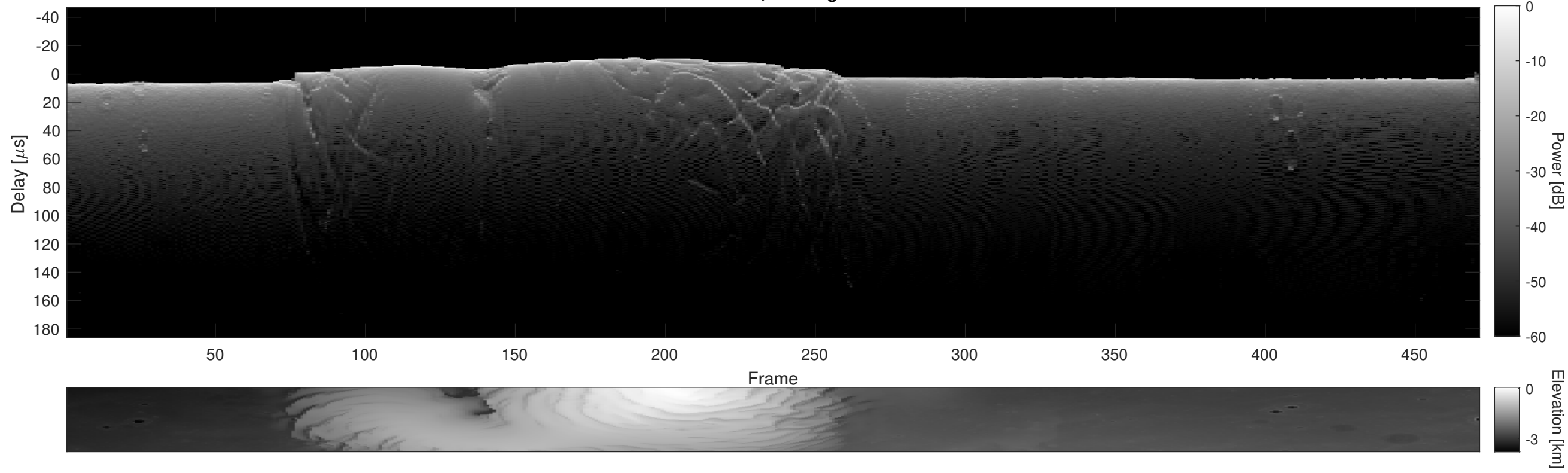
Orbit 5424, Cluttergram
